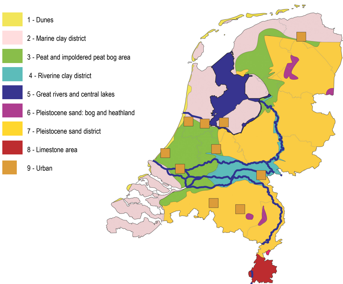
Fig 11. Classification of regions based on physical-chemical and physical-geographical parameters (see table 5).
